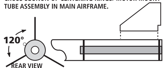
CROSS SECTION OF CENTERING RINGS/ MOTOR MOUNT TUBE ASSEMBLY IN MAIN AIRFRAME.
